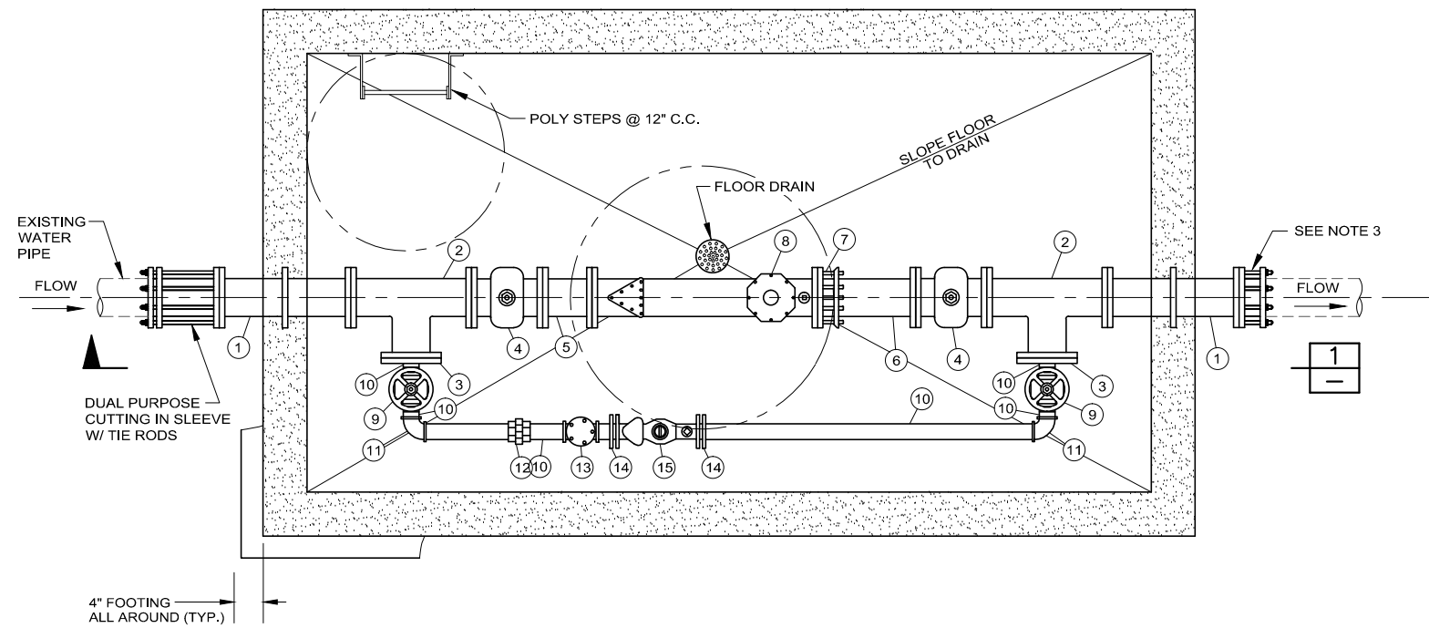
10" METER STATION PLAN NOT TO SCALE
